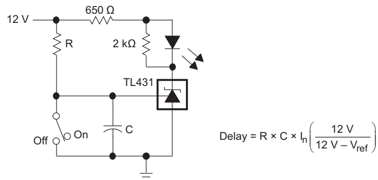
Figure 37. Delay Timer
